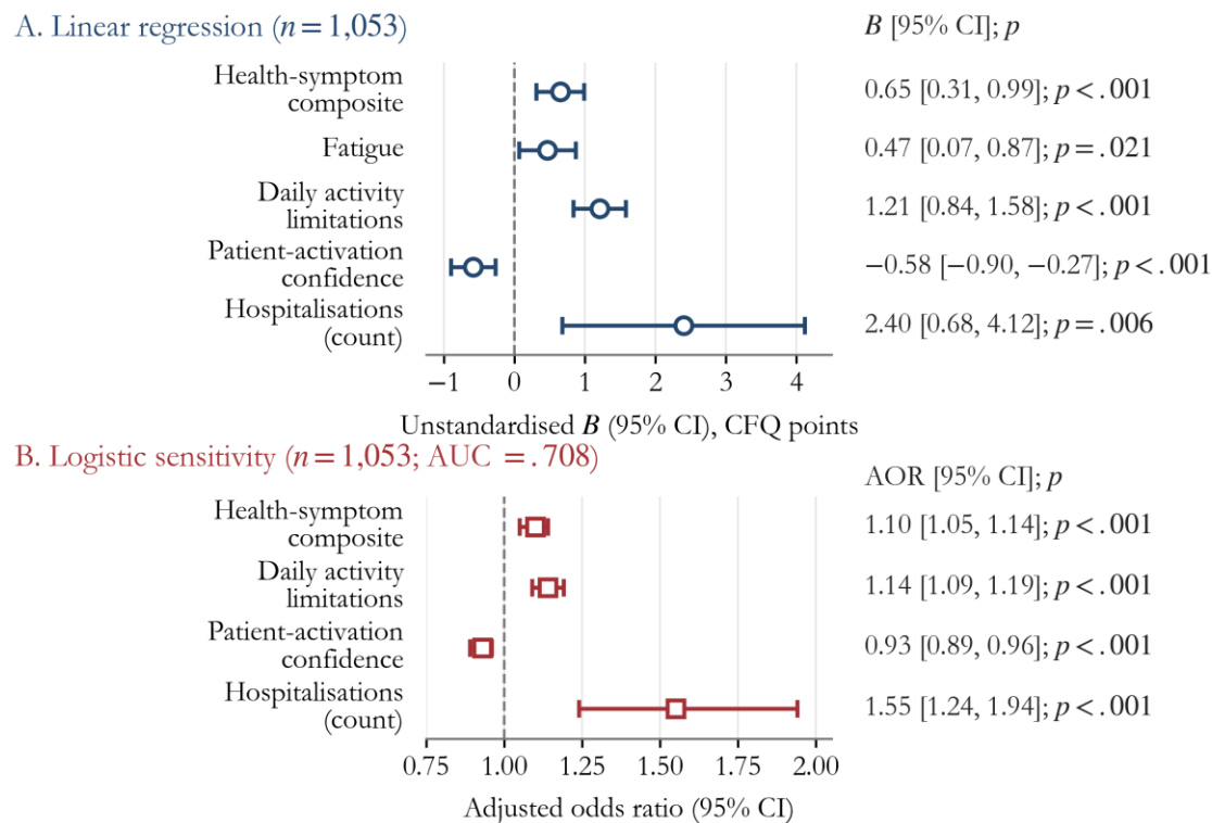
Figure 2. Adjusted associations with self-reported cognitive failures (CFQ). A. Linear regression of continuous CFQ ( n = 1,053 ). B. Logistic sensitivity analysis for High CFQ > 32 ( n = 1,053 ; AUC = .708). Error bars = 95% CIs. Coefficients are unstandardised; predictors are on different scales
